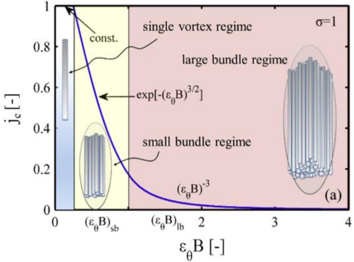
Figure 1.6. The J_c(B) pinning regimes as collective pinning theory [56]
