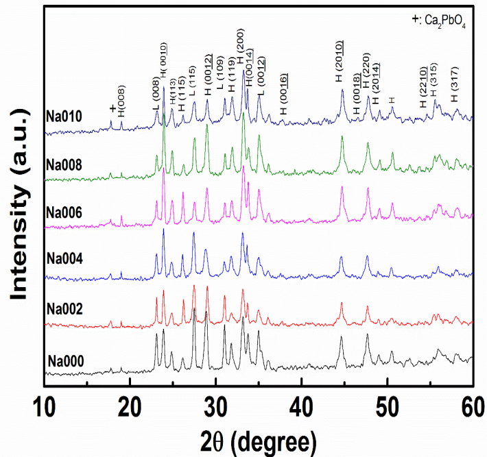
Figure 3.1. XRD patterns of \text{Bi}_{1.6}\text{Pb}_{0.4}\text{Sr}_2\text{Ca}_{2-x}\text{Na}_x\text{Cu}_3\text{O}_{10+\delta} samples [109]
