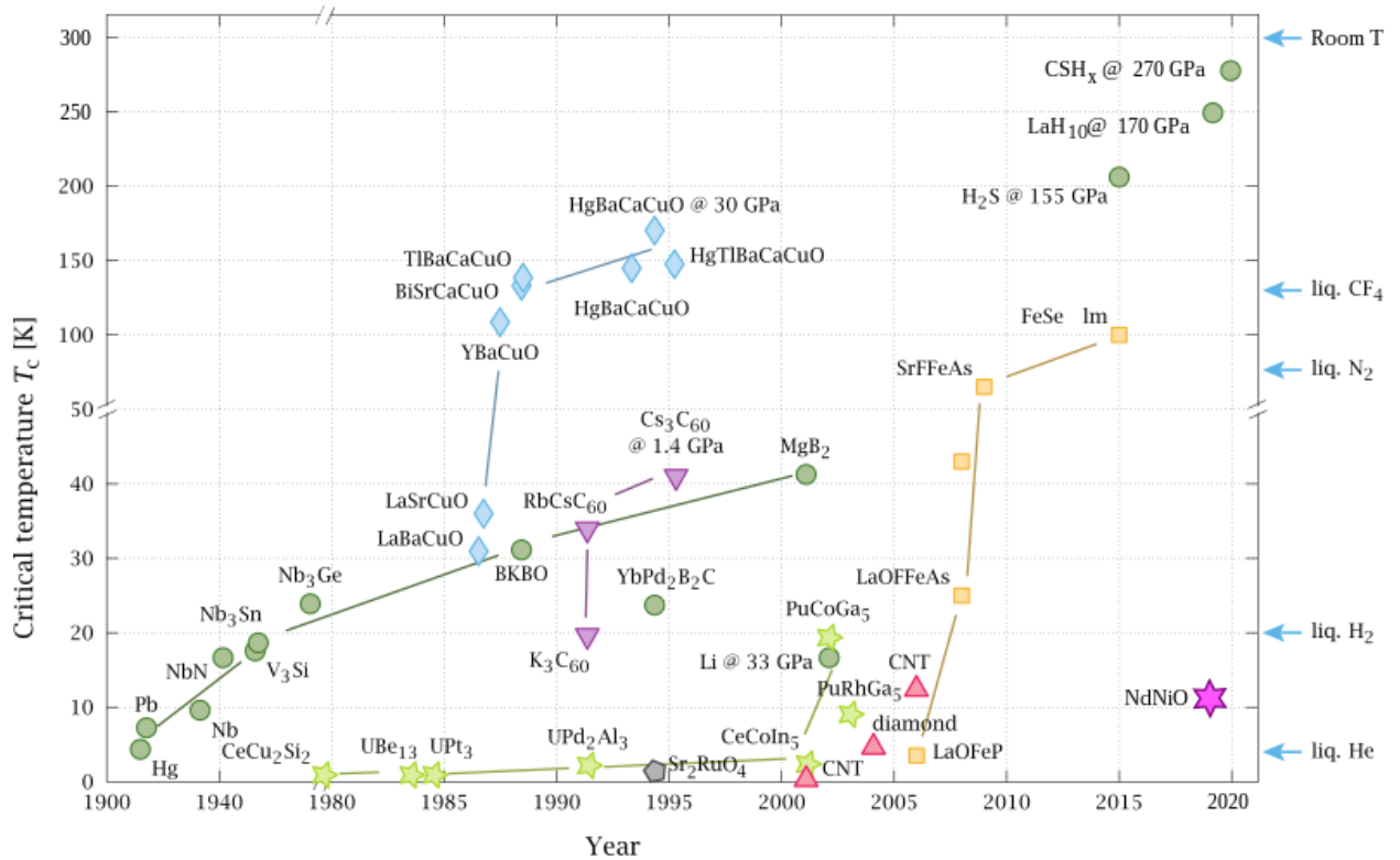
Figure 1.1. History of Superconductivity [95]
