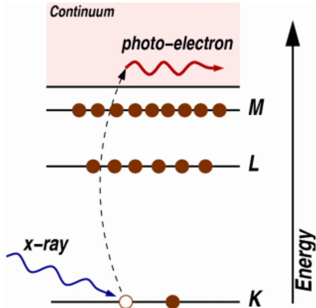
Figure 2.3. The photoelectric effect, in which an x-ray is absorbed and a core level electron is promoted out of the atom [75]
