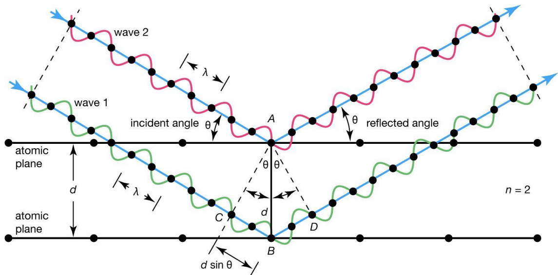
Figure 2.2. Bragg's Law reflection [134]
