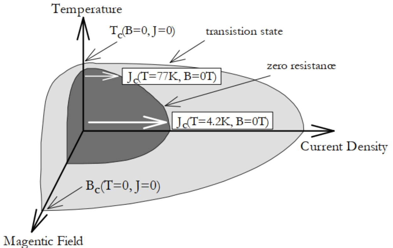
Figure 1.2. Three states of conductivity in a superconductor: zero resistance (inside the innermost surface), transition state (outer surface), and normal conductance (beyond the outer surface) [76]
