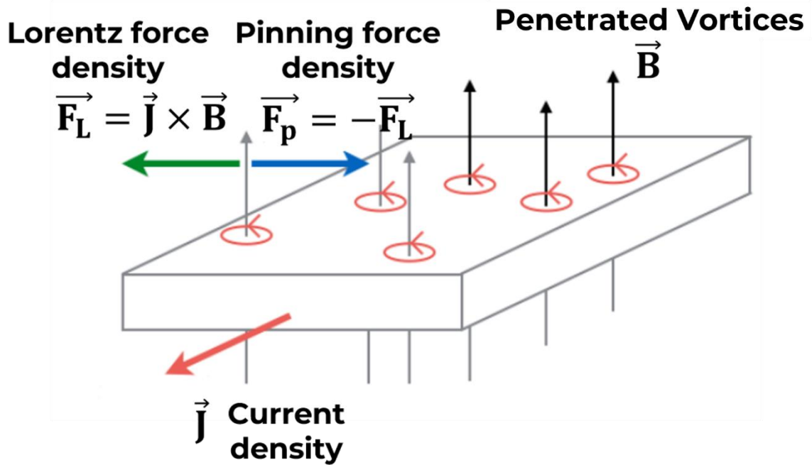
Figure 1.7. Balance of forces acting on vortices [103]
