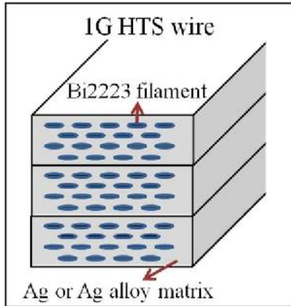
Figure 1.11. BSCCO 1 st generation HTS wire [44]
