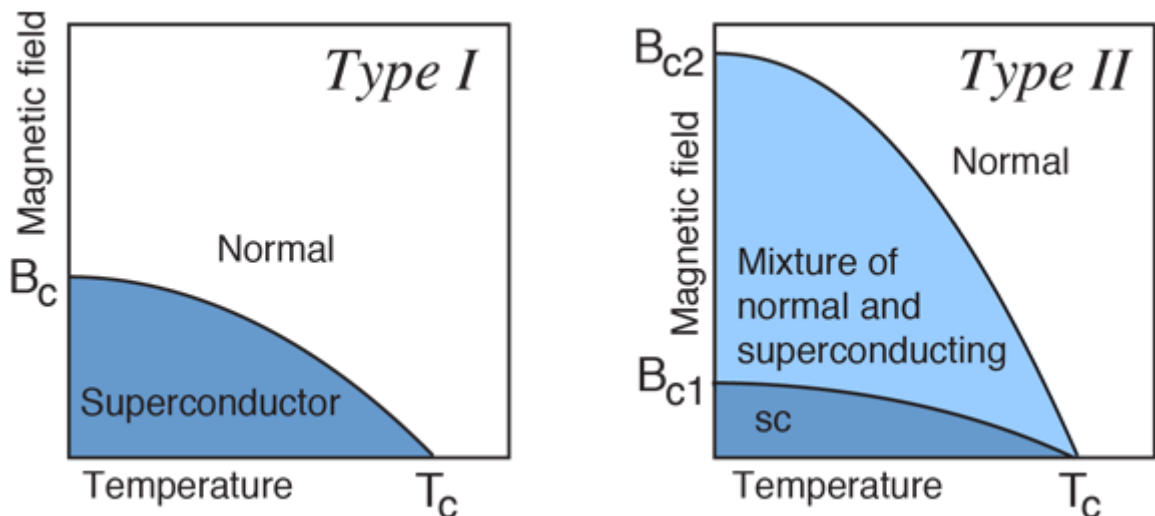
Figure 1.3. Phase diagram of Type-I and Type-II superconductors [97]
