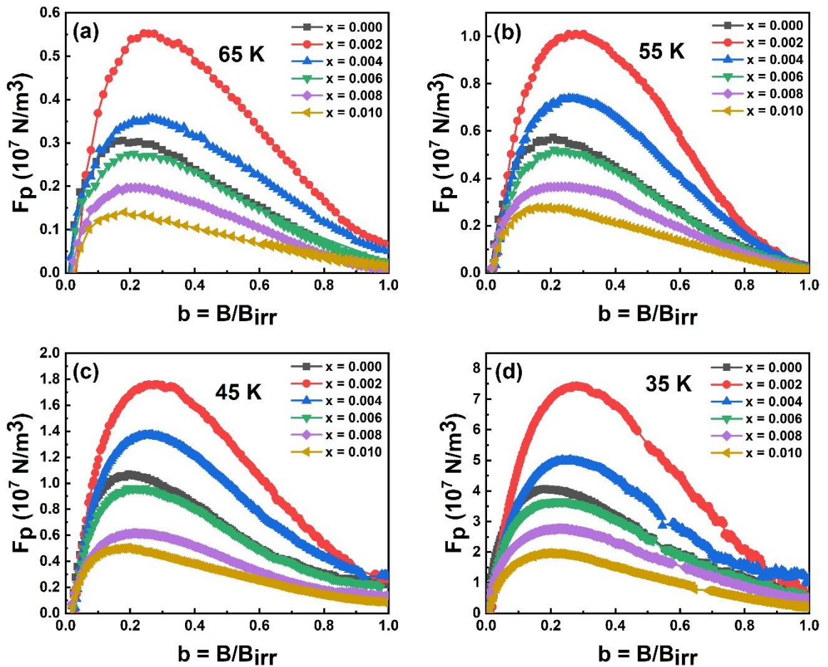
Figure 4.12. The normalized field dependence of flux pinning force density of (Bi_{1.6}Pb_{0.4}Sr_2Ca_2Cu_3O_{10+\delta})_{1-x}(TiO_2)_x samples, with x = 0, 0.002, 0.004, 0.006, 0.008, and 0.010 at (a) 65 K, (b) 55 K, (c) 45 K, and (d) 35 K
