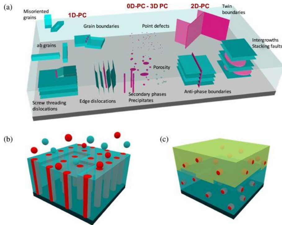
Figure 1.8. Schematic of different types of nano-sized pinning centers in type-II superconductors [85]
